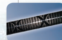
Multi layer hi-modulus/hi-density carbon blank with double X hi-resistance carbon reinforcement.
